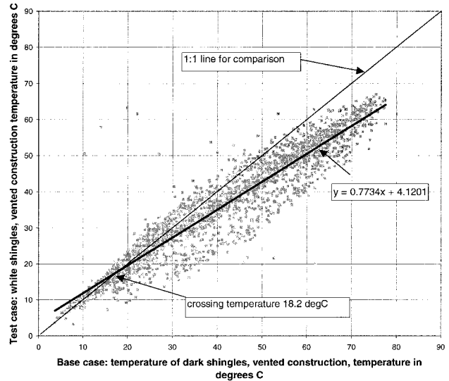
Figure 4 Illustration of linear regression method that uses comparison of test case values against a base case. In this example, the temperature at the underside of white shingles (vented attic) is compared to the temperature at the underside of dark shingles (vented attic). The slope of the regression line is 0.773, so the white shingles are 22.7% cooler ( 1 - 0.773 ).
