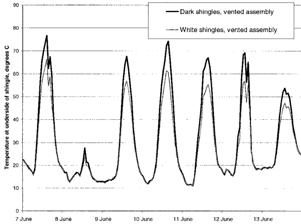
Figure 3 Sample measured temperature data for two conditions: (1) underside of dark shingles, ventilated attic, and (2) underside of white shingles, ventilated attic.
