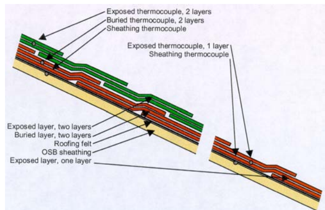
Figure 2 Schematic diagram showing shingles and thermocouple placement, bays 1, 3, and 4. Note that the thermocouple placement called “sheathing” represents the top of the sheathing as well as the underside of the felt. The “sheathing” location represents the sheathing/roof material interface.
